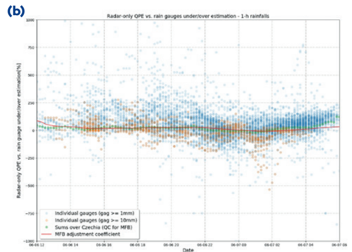
Fig. 6.4 Example of radar under/over estimation variability for 6 days from June 3, 2019 to June 9, 2019 (a), and a detailed view of variability over 18-hour period from June 6, 2019 12:00 UTC to June 7, 2019 06:00 UTC (b). Examples depict one of the episodes with selected significant FFI cases of intense convective rainfall (as explained in Chapter 6.1.3). Intense rainfalls with FFI response were identified from June 4, 2019 to June 6, 2019.
