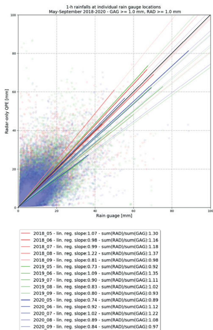
Fig. 6.2 Comparison of 1-hour rain gauge rainfalls and radar-only estimates at individual rain gauge locations during May–September 2018–2020.
