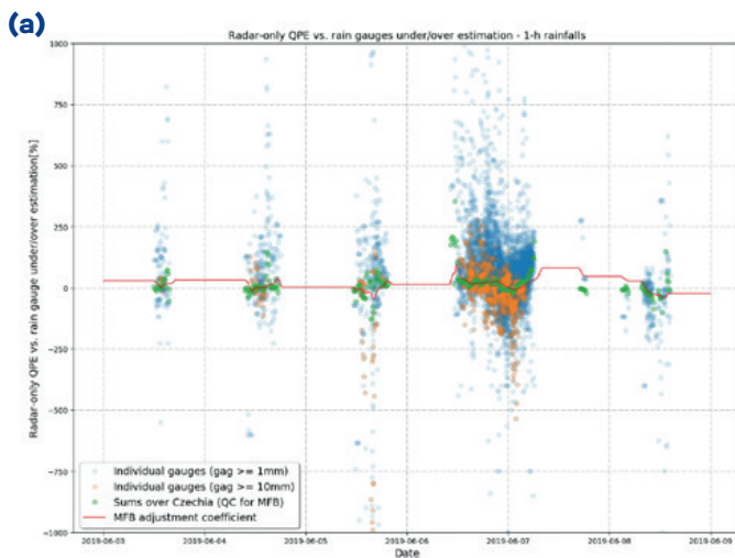
Fig. 6.4 Example of radar under/over estimation variability for 6 days from June 3, 2019 to June 9, 2019 (a), and a detailed view of variability over 18-hour period from June 6, 2019 12:00 UTC to June 7, 2019 06:00 UTC (b). Examples depict one of the episodes with selected significant FFI cases of intense convective rainfall (as explained in Chapter 6.1.3). Intense rainfalls with FFI response were identified from June 4, 2019 to June 6, 2019.
